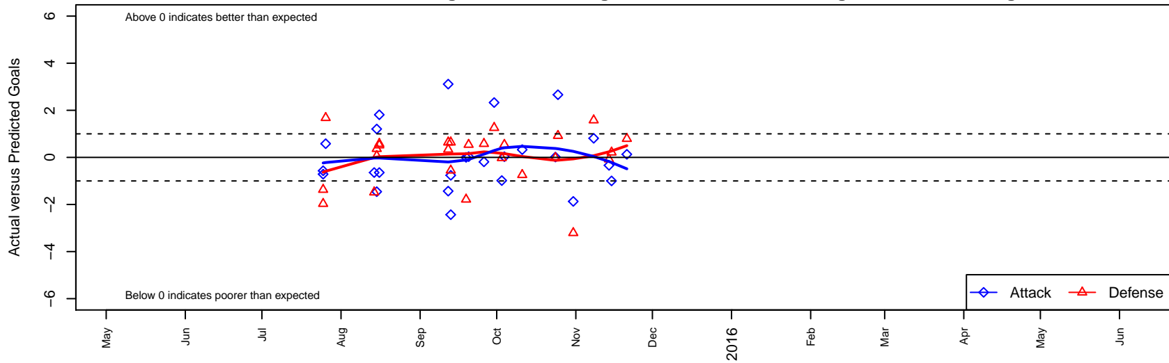
Breakers Black 2001B Dots are actual minus expected GF (blue circles) and GA (red triangles). Blue line is smoothed change in attack strength. Red is smoothed change in defense strength.
